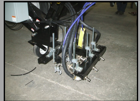
Rebuilt KC-700SS Paint Guns Rebuilt Binks Model 30 Bead Guns
