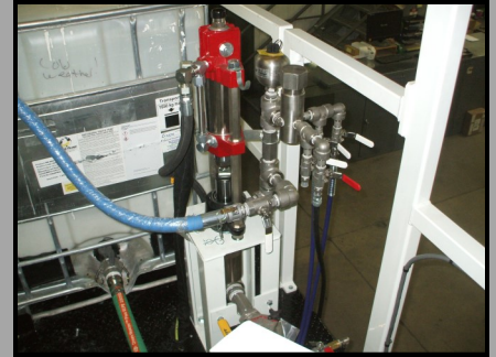
Titan/SpeedFlo 8.6 GPM Airless Paint Pumps
